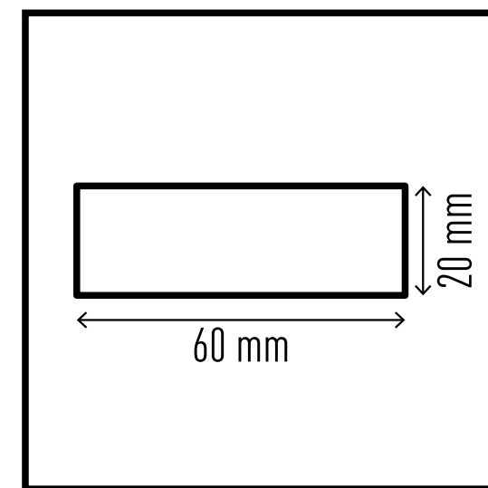
Surface protection profile S20 #1108-130
