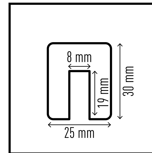
Edge protection profile E8 #1127-130
