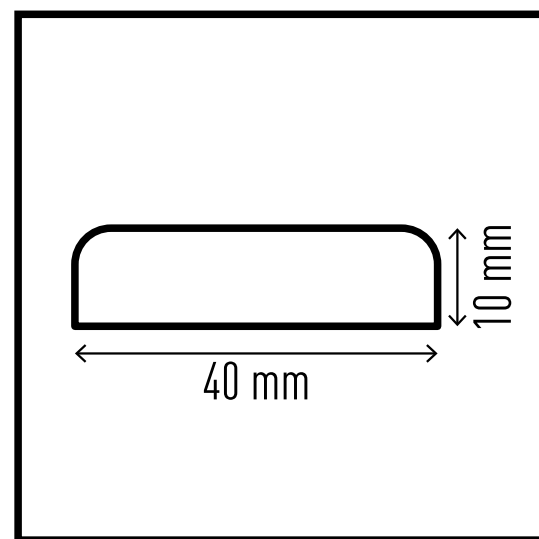
Surface protection profile S10 #1107-130
