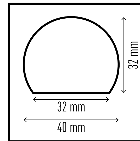
Surface protection profile S32R #1109-130
