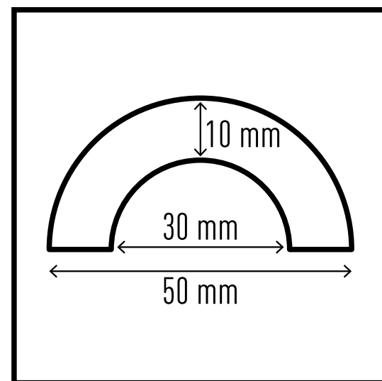
Pipe protection profile P30 #1115-130
