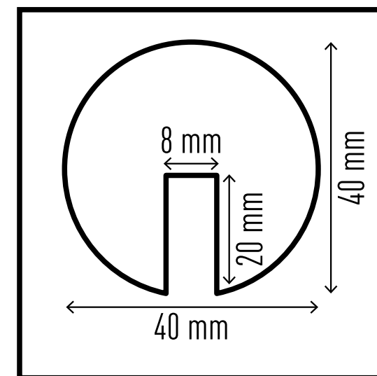
Edge protection profile E8R #1126-130
