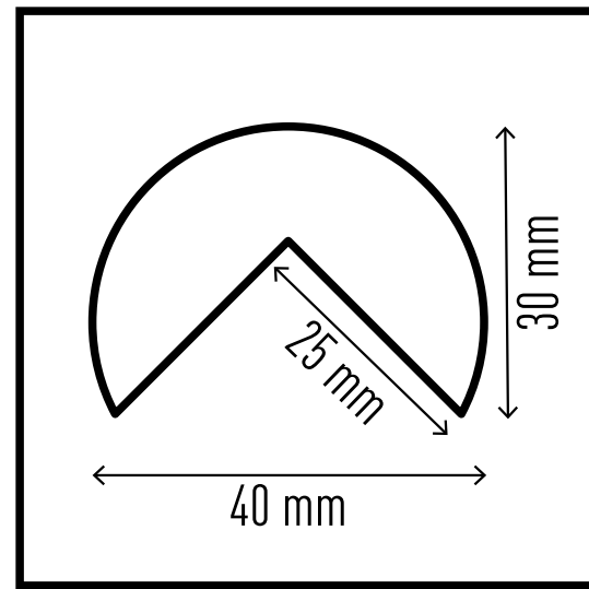
Corner protection profile C25R #1100-130 / #1110-130
