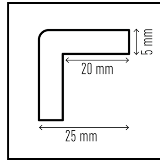
Corner protection profile C20 #1101-130 / #1111-130
