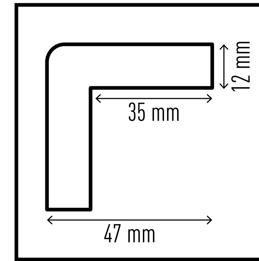
Corner protection profile C35 #1102-130 / #1112-130
